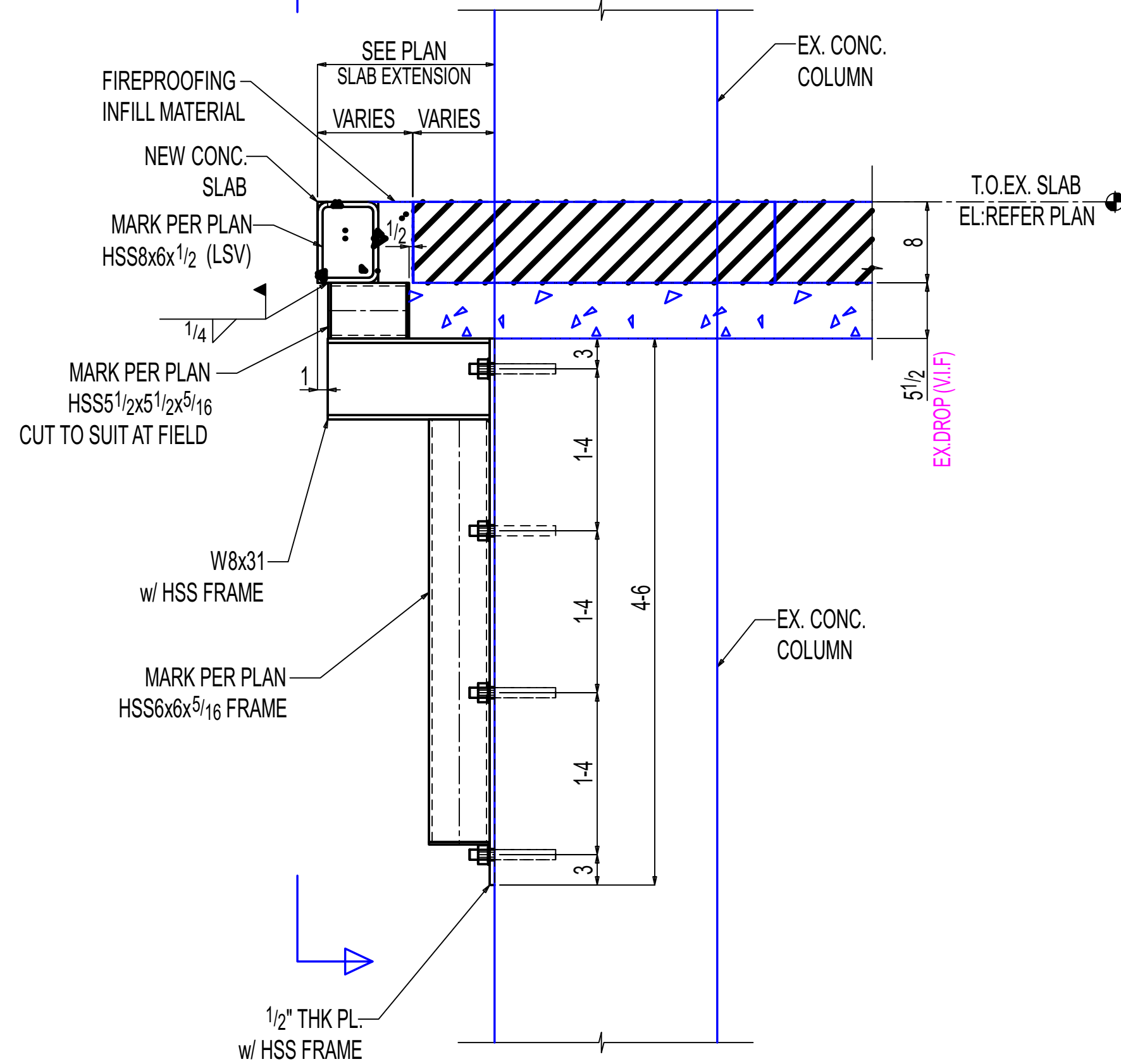
D-D ( NEW SLAB EXTENSION SUPPORT @ SLAB DROP LOCATION NEW SLAB EXTENSION BETWEEN 1'-0" TO 1'-6" ) E-13.00 (REF:10 & 11/S314) OTHERS NOT SHOWN FOR CLARITY
